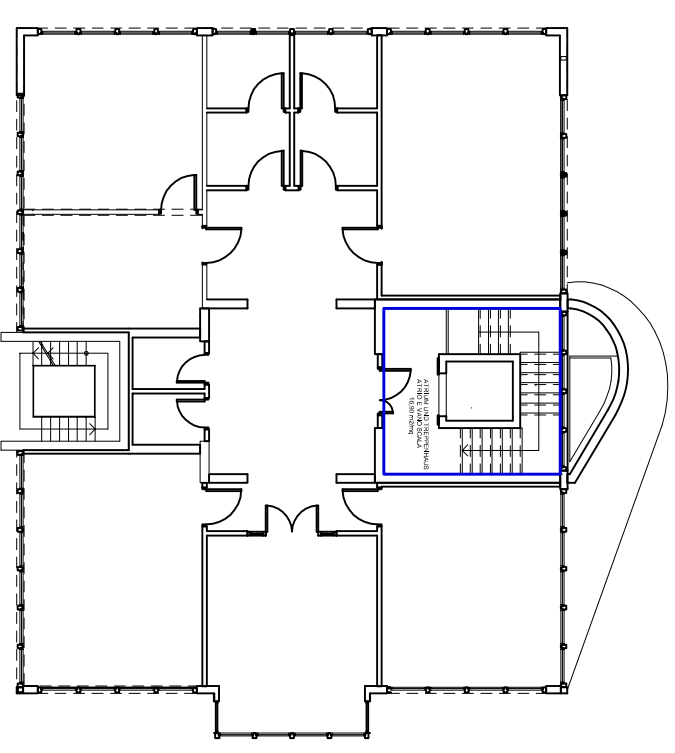
GRUNDRISS 2. OBERGESCHOSS PIANTA 2° PIANO
